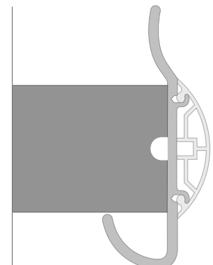
Reverse hook assembly height 145 depth 114mm
