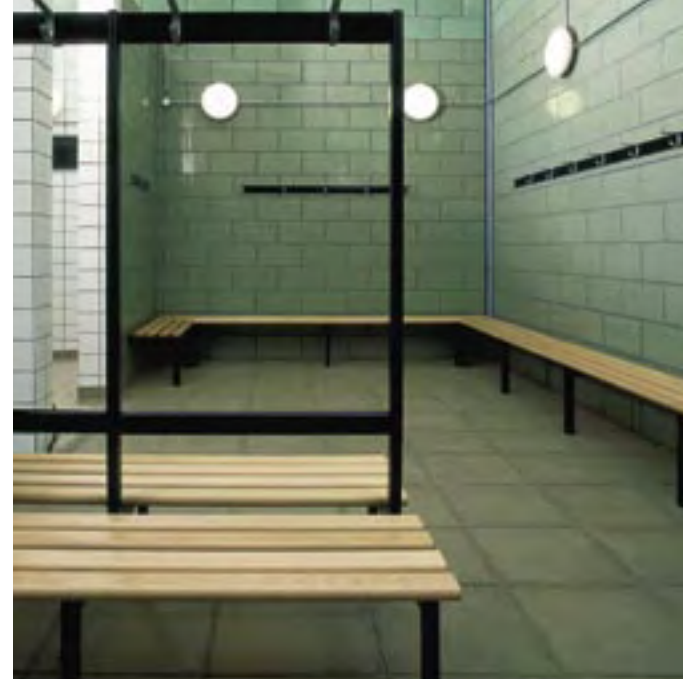
code VZ1-4 island unit with hooks, bench seat and backrest code VZ7-4 units around the walls
